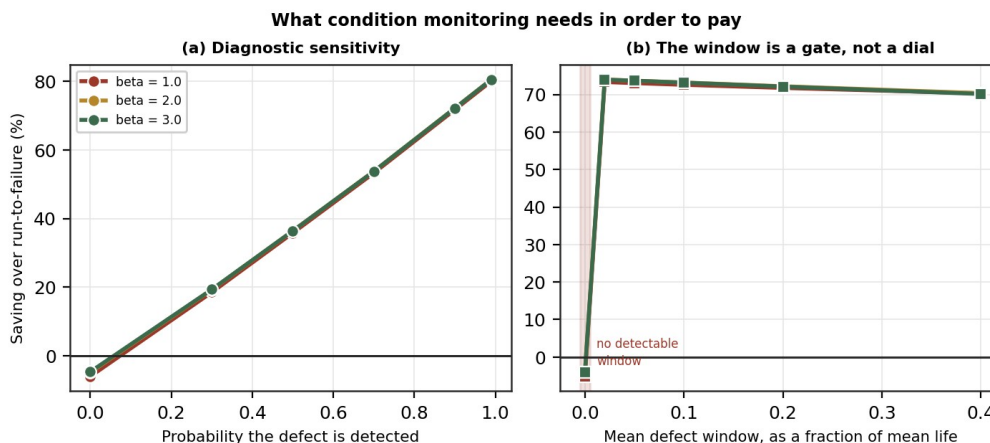
Fig.4: Condition-based saving against detection probability and against the defect window.
