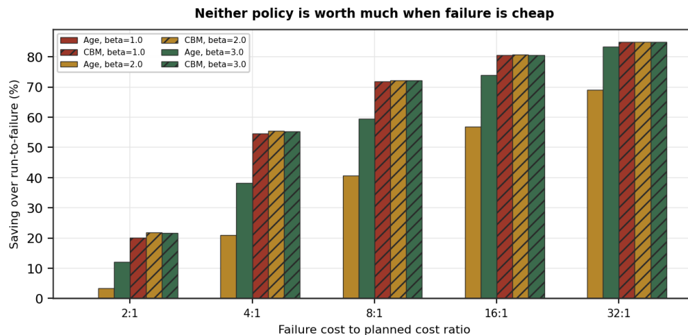
Fig.6: Saving against the failure-to-planned cost ratio for both policies.
