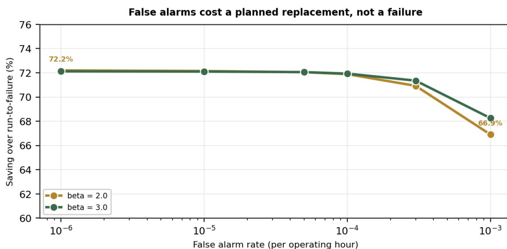
Fig.5: Saving against false alarm rate.
