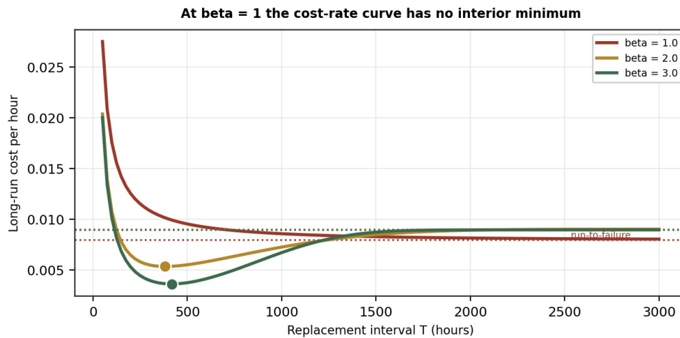
Fig.2: Cost rate against replacement interval. At \beta = 1 there is no interior minimum.
