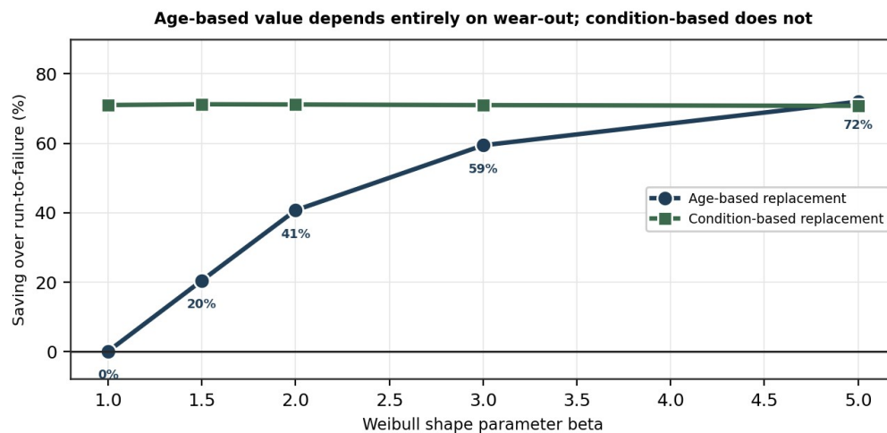
Fig.3: Saving over run-to-failure for both policies against the shape parameter.
