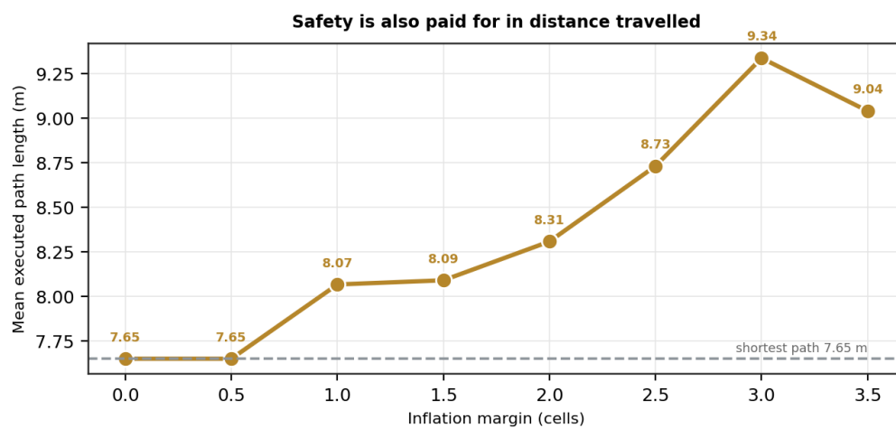
Fig.6: Mean executed path length against inflation margin.
