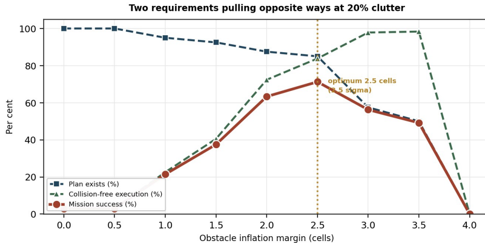
Fig.2: Planning success, collision-free execution and their product against inflation margin.
