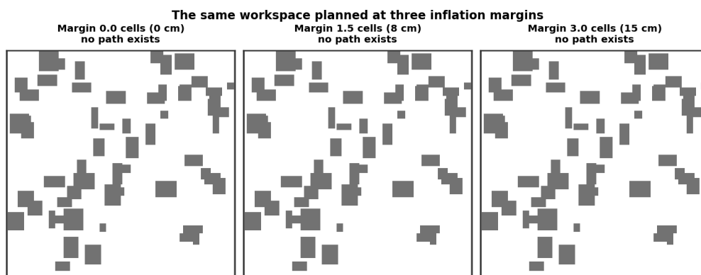
Fig.1: One workspace planned at three inflation margins. At the largest margin no route survives.
