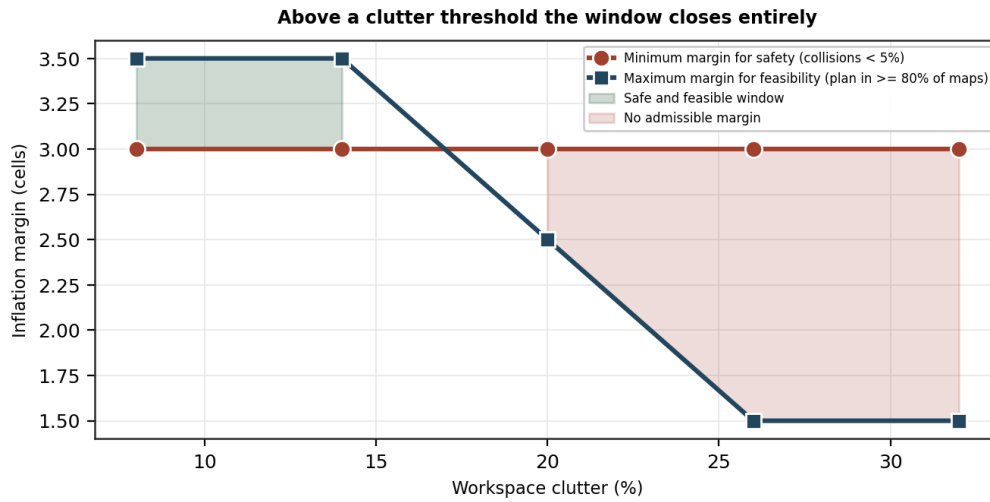
Fig.4: The safety requirement and the feasibility ceiling against clutter.
