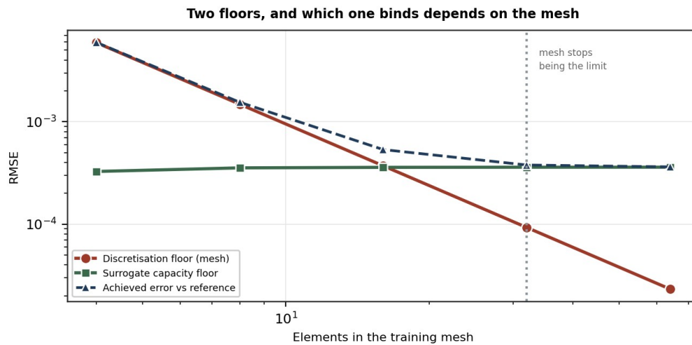
Fig.5: The discretisation floor, the surrogate capacity floor, and the error achieved.
