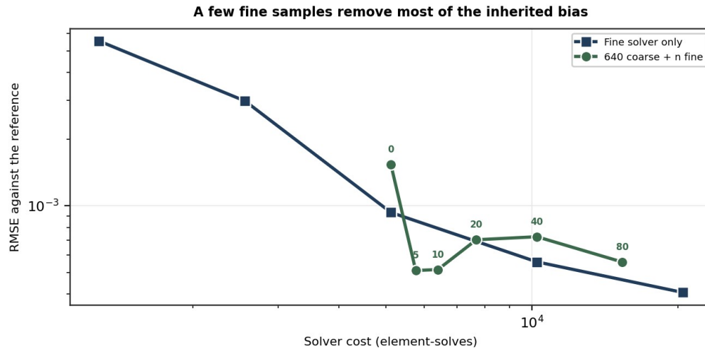
Fig.6: Multi-fidelity correction against a matched-cost single-fidelity baseline.
