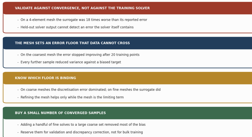
Fig.7: Proposed practice for building and reporting simulation surrogates.
