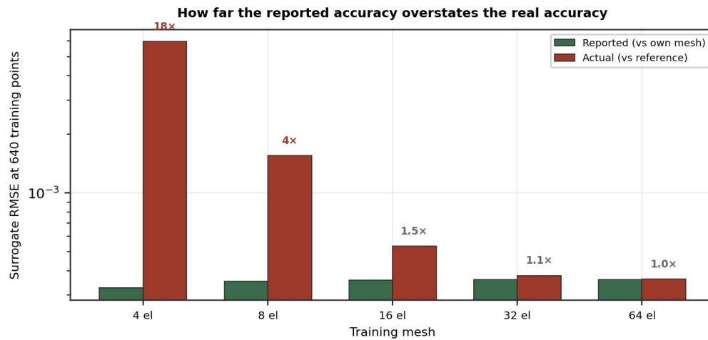
Fig.4: Reported and actual surrogate error at the largest training-set size.
