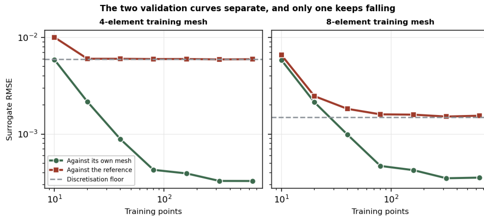
Fig.3: Learning curves scored against the training mesh and against the reference.
